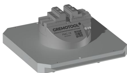
PMC-74 & System 3R Delphin 398 Pallet
