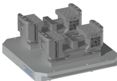
2x SC-100 & System 3R Delphin 398 Pallet
