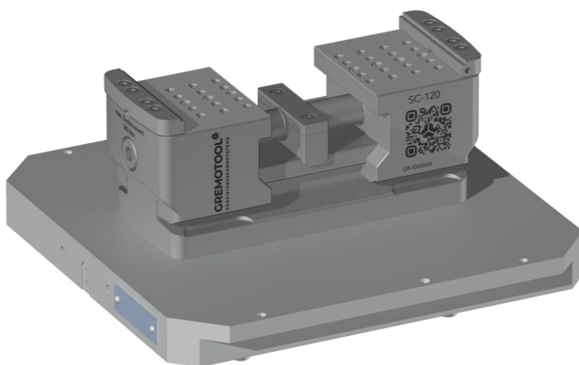
SC-120 & System 3R Delphin 398 Pallet
