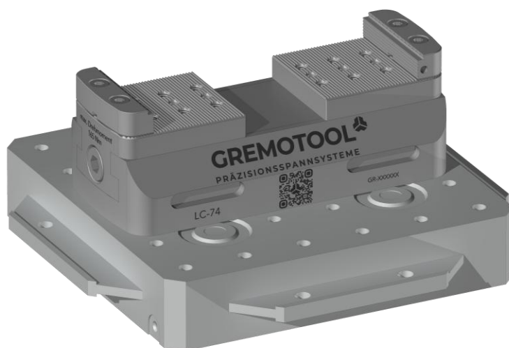
LC-74 & System 3R GPS-240 Pallet
