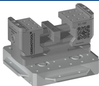
SC-100 & System 3R GPS-240 Pallet
