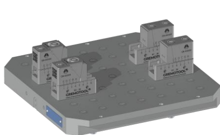
2x RC-38 & System 3R Delphin 398 Pallet
