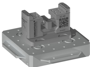
SC-60 & System 3R GPS-240-Pallet
