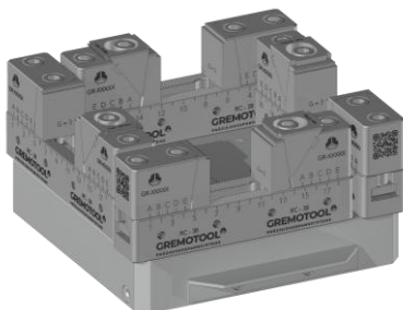
4x RC-38 & System 3R GPS-240 Pallet
