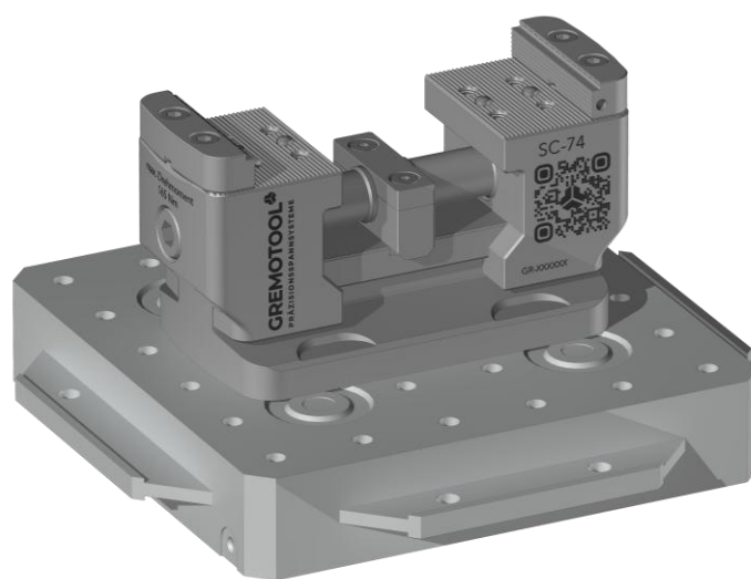
SC-74 & System 3R GPS-240 Pallet
