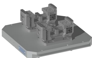
2x SC-74 & System 3R Delphin 398 Pallet
