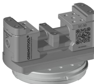
SC-50 & System 3R GPS-120 Pallet
