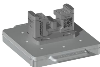
SC-60 & System 3R Dynafix Pallet
