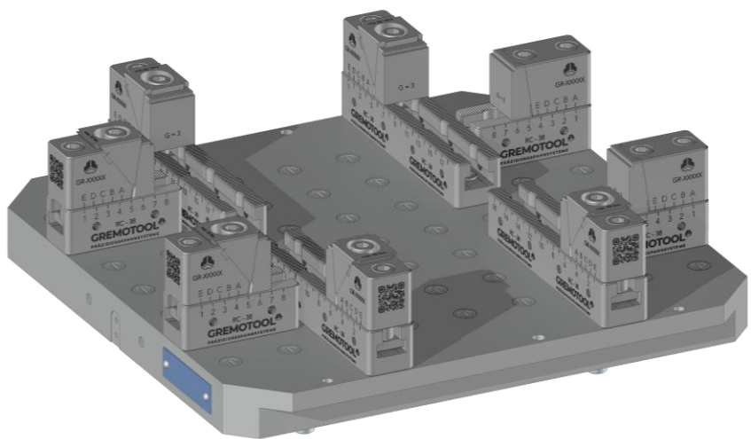
4x RC-38 & System 3R Delphin 398 Pallet
