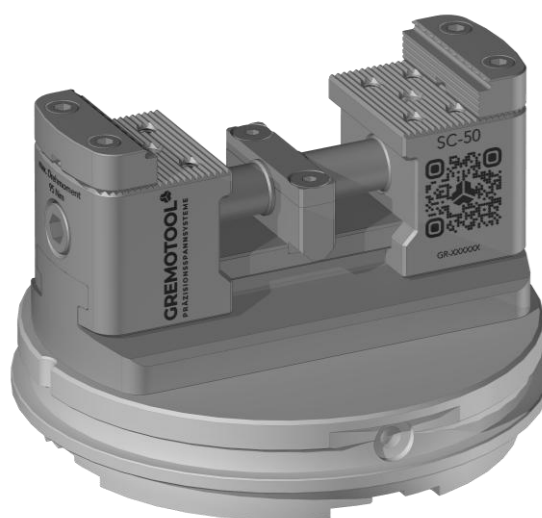
SC-50 & System 3R MacroMagnum Pallet
