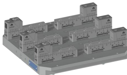
3x RC-38 & System 3R Delphin 448 Pallet
