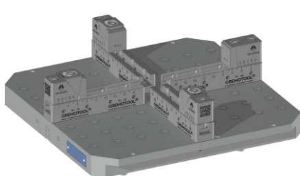
2x RC-38 & System 3R Delphin 448 Pallet
