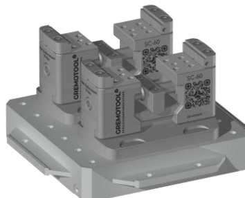
2x SC-60 & System 3R GPS-240 Pallet
