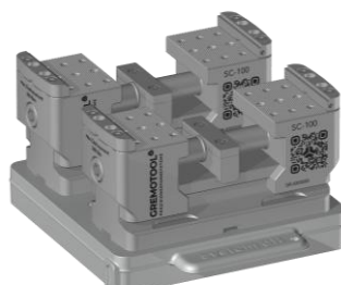
2x SC-100 & System 3R Dynafix Pallet
