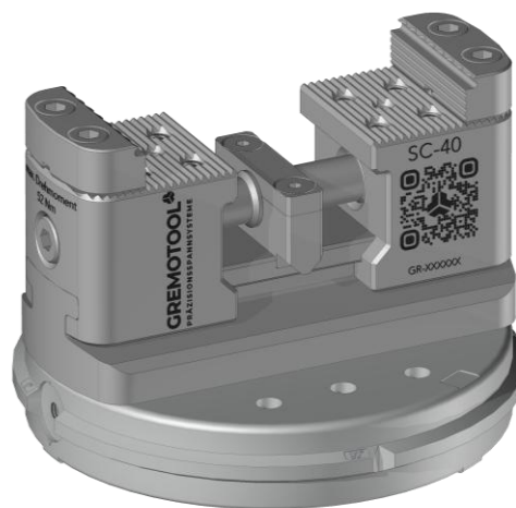
SC-40 & System 3R GPS-120 Pallet
