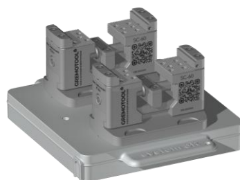
2x SC-60 & System 3R Dynafix Pallet
