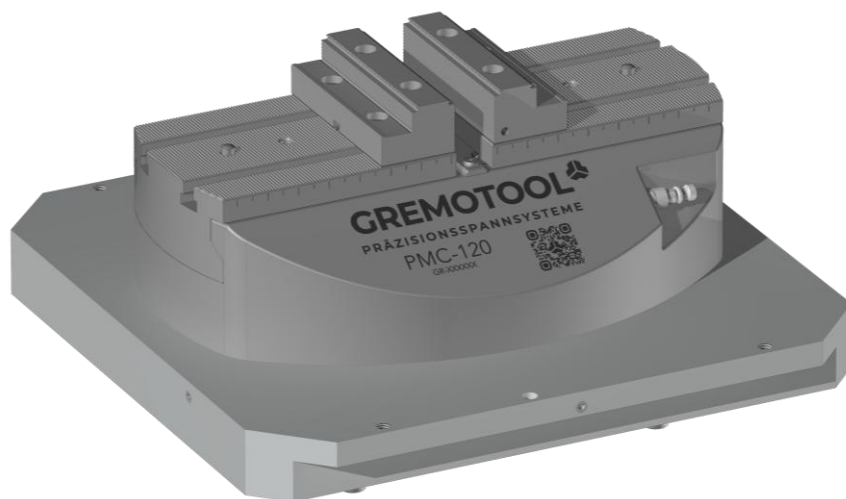
PMC-120 & System 3R Delphin 398 Pallet
