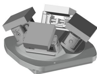
4x SC-50 con Piramide & System 3R Dynafix Pallet
