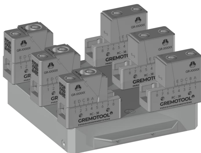
3x RC-38 & System 3R GPS-240 Pallet
