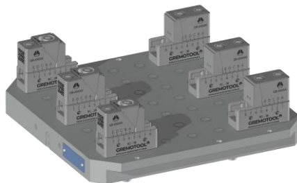
3x RC-38 & System 3R Delphin 398 Pallet
