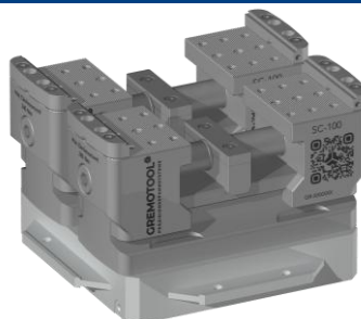
2x SC-100 & System 3R GPS-240 Pallet
