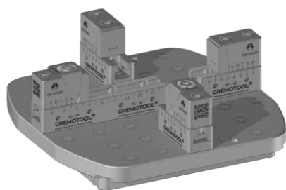
2x RC-38 & System 3R Dynafix Pallet
