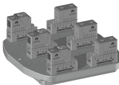
3x RC-38 & System 3R Dynafix Pallet
