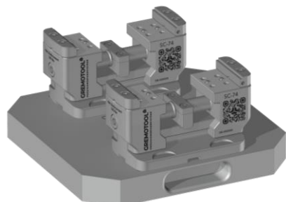
2x SC-74 & Erowa UPC-320-Pallet
