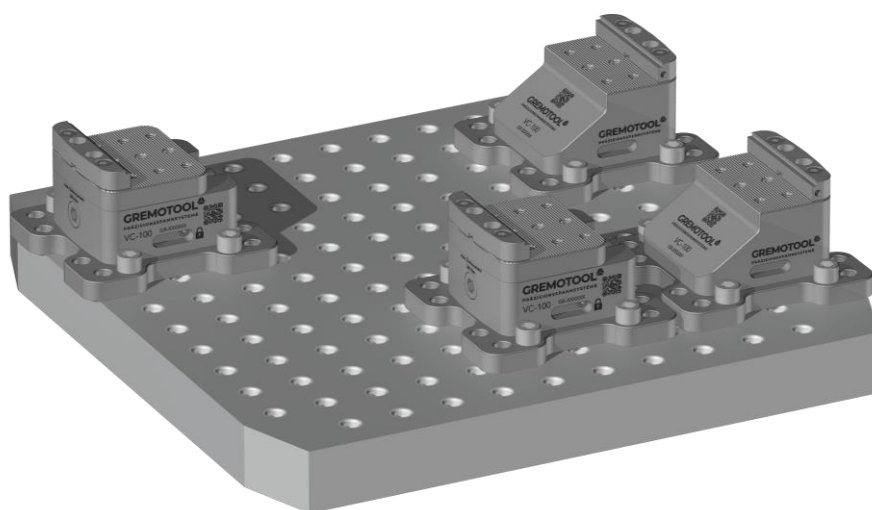
2x VC-100 & Erowa MTS-498 Pallet
