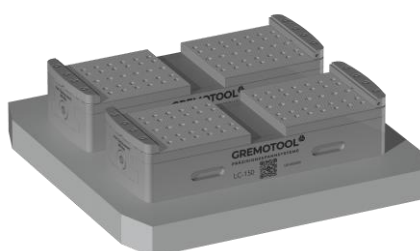
2x LC-150 & Erowa MTS-498 Pallet
