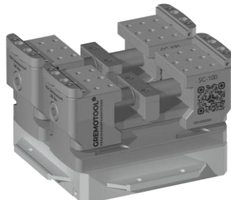
2x SC-100 & System 3R GPS-240 Pallet
