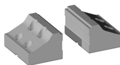
Gripper jaw high one-sided Nr. 837380-BXX
